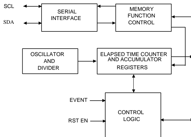
DS1676 Block Diagram Figure 1
