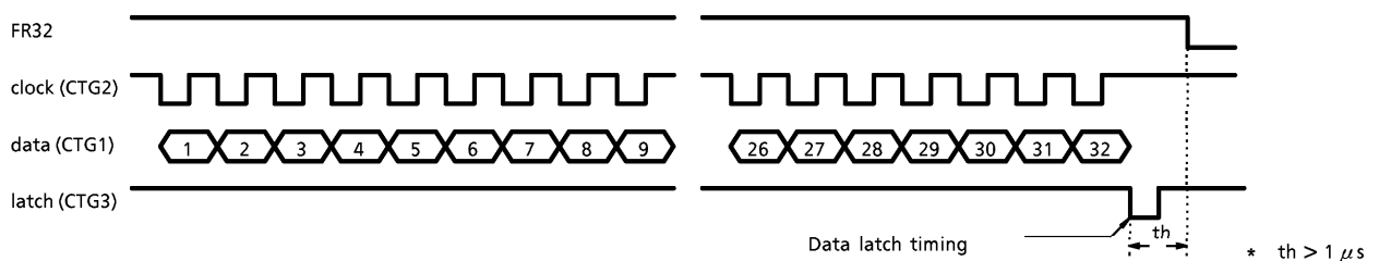
Figure 7 Serial Interface Timing Example
