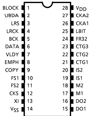
TC9271F, TC9271N
