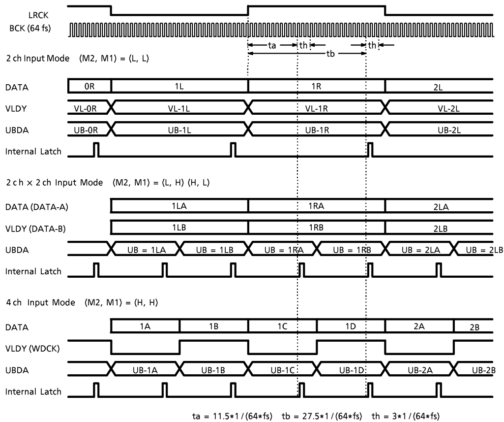
Figure 2 V and U Bit Input Timing Chart
