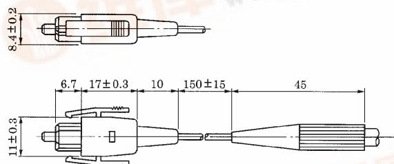
(2) Optical fiber
