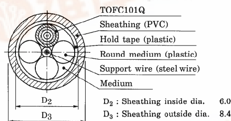
(2) Optical fiber
