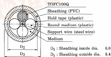
(2) Optical fiber
