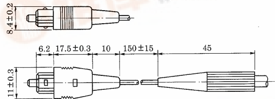
(1) Fiber optic connector
