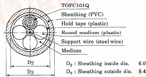
(2) Optical fiber
