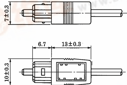
(1) Fiber optic connector
