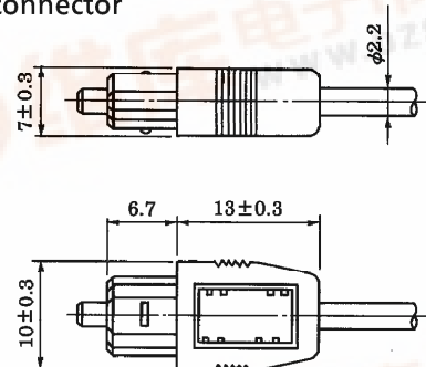
(1) Fiber optic connector
