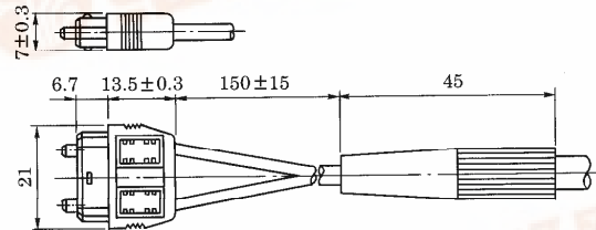
(2) Optical fiber
