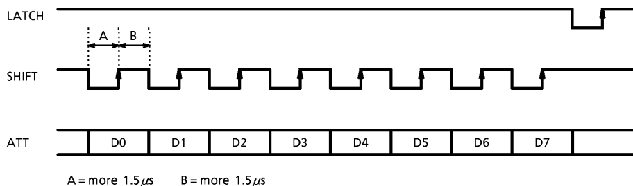
Fig.10 Example for serial control mode data
