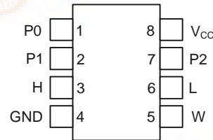
8-Pin DIP (300-mil)
