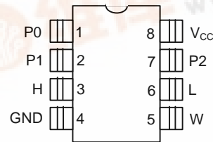
8-Pin SOIC (150-mil)
