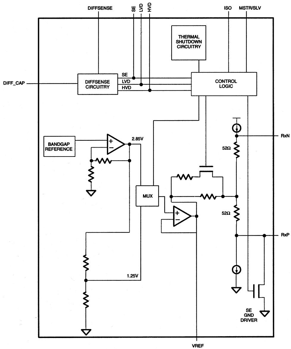
DS2120A BLOCK DIAGRAM Figure 1
