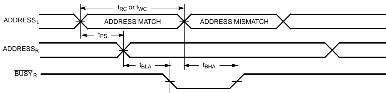
Busy Timing Diagram No. 2 (Address Arbitration) [36]
