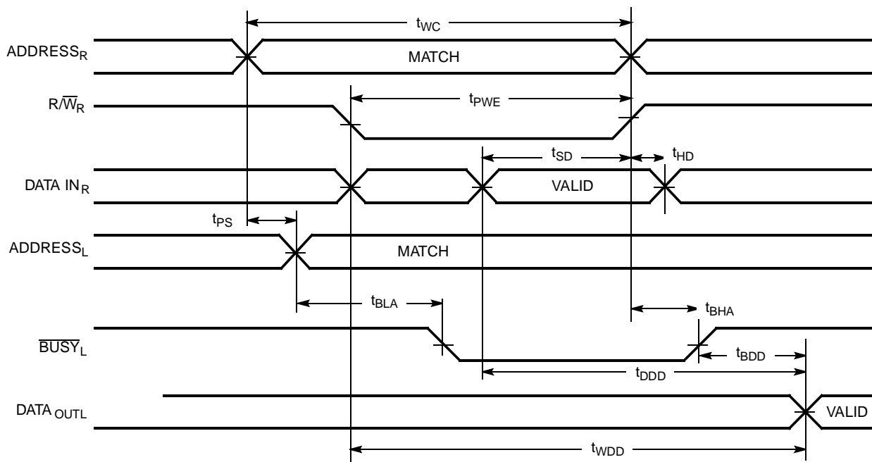
Timing Diagram of Read with \overline{\text{BUSY}} ( M/\overline{\text{S}}=\text{HIGH} ) [35]
