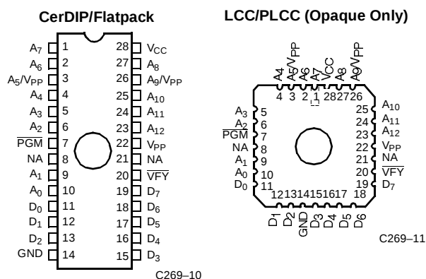
Figure 1. Programming Pinouts
