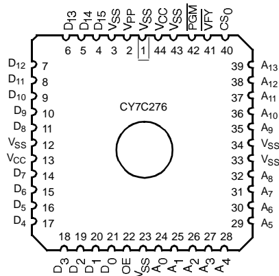
Figure 1. Programming Pinout
