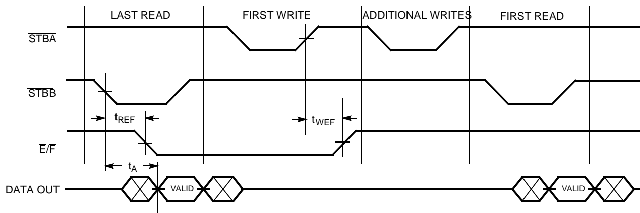
Last Read to First Write Empty/Full Flag Timing Diagram [11]
