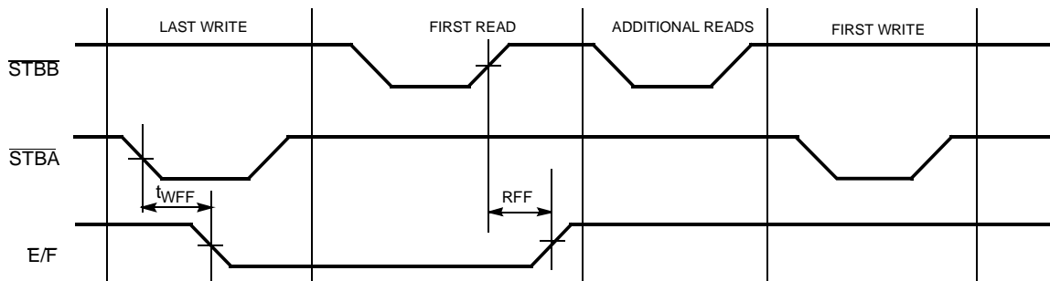
Last Write to First Read Empty/Full Flag Timing Diagram [11]
