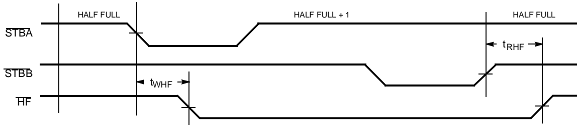
Half-Full Flag Timing Diagram [11]
