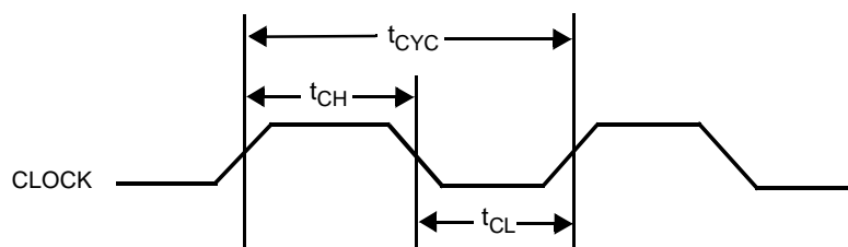
Figure 21-1. Clock Timing
