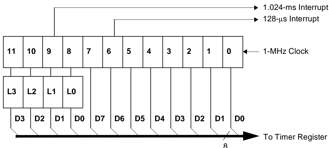
Figure 10-3. Timer Block Diagram
