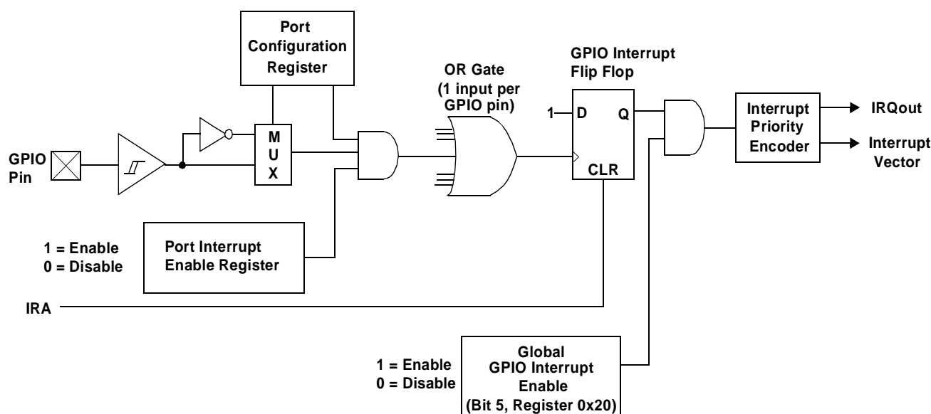
Figure 14-5. GPIO Interrupt Structure
