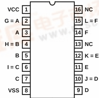
CD4050BMS TOP VIEW
