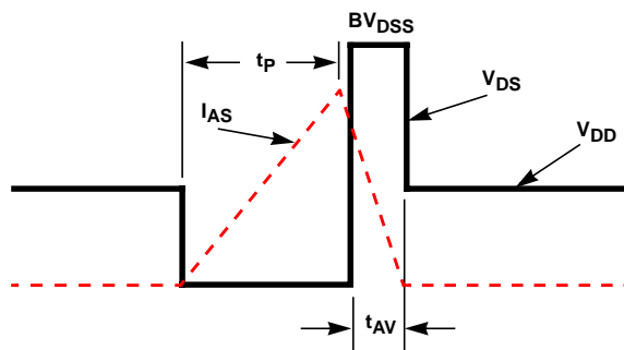
FIGURE 10. UNCLAMPED ENERGY WAVEFORMS
