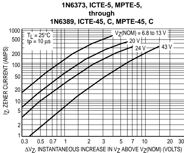
Figure 6. Dynamic Impedance
