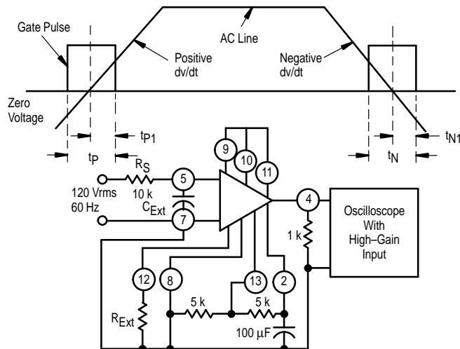
Figure 6. Gate Pulse Duration Test Circuit with Associated Waveform
