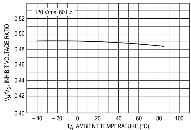
Figure 13. Inhibit Voltage Ratio versus Ambient Temperature
