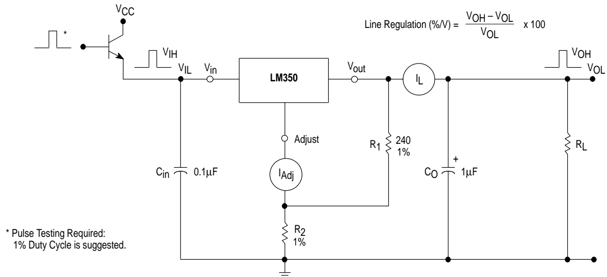
Figure 1. Line Regulation and \Delta I_{Adj}/Line Test Circuit
