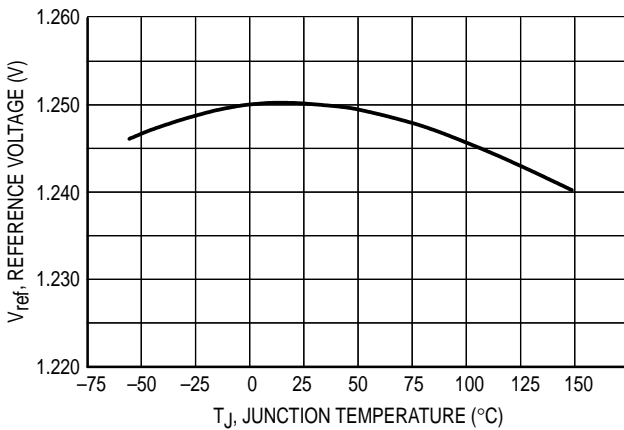
Figure 9. Temperature Stability
