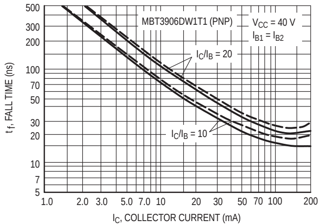
Figure 24. Fall Time
