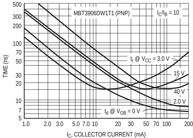
Figure 23. Turn-On Time
