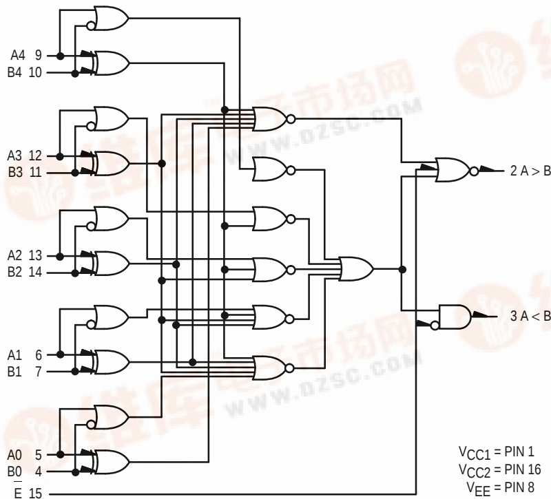
LOGIC DIAGRAM
