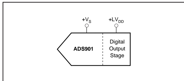
FIGURE 7. Independent Supply Connection for Output Stage.
