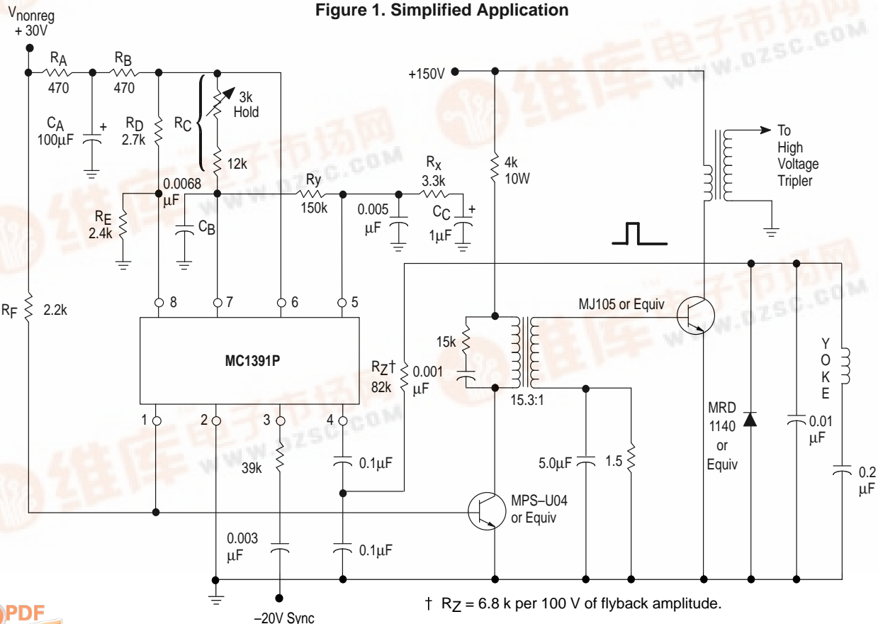
Figure 1. Simplified Application
