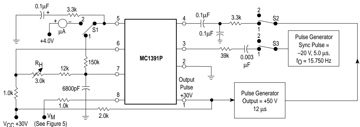
Figure 2. Test Circuit
