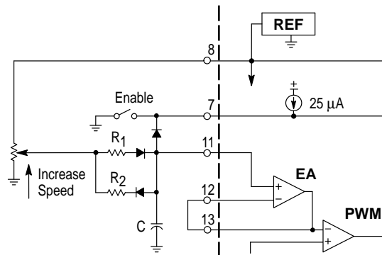
Figure 32. Controlled Acceleration/Deceleration
