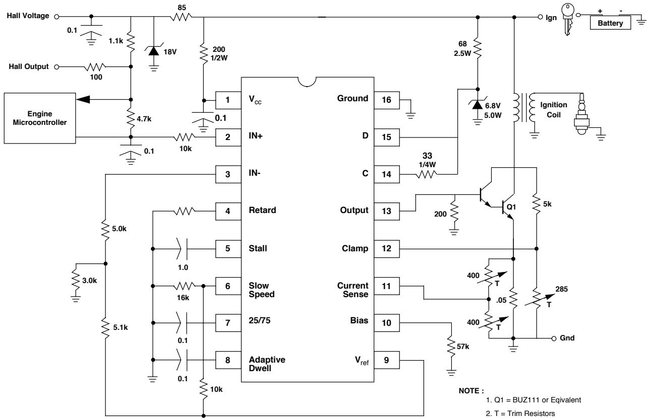
Figure 3. Application Circuit (Hall Sensor Input)
