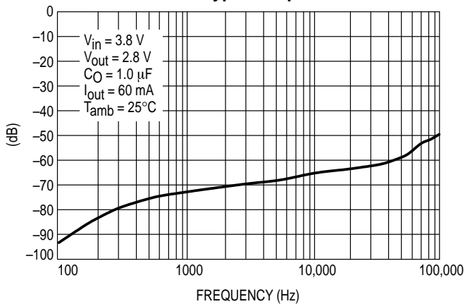
Figure 19. Ripple Rejection versus Frequency with 10 nF Bypass Capacitor
