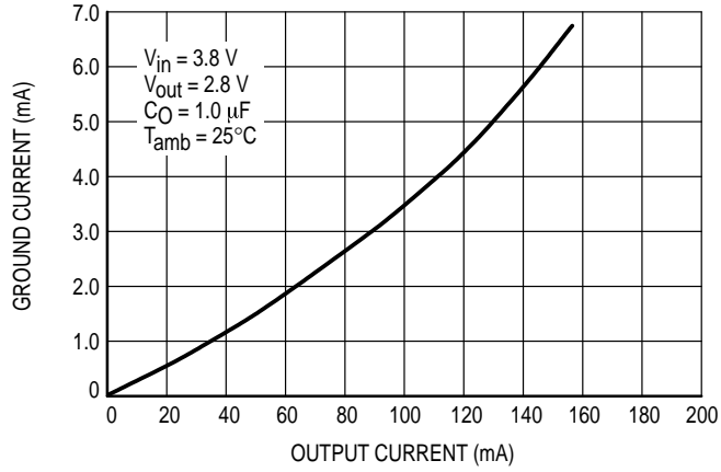
Figure 1. Ground Current versus Output Current
