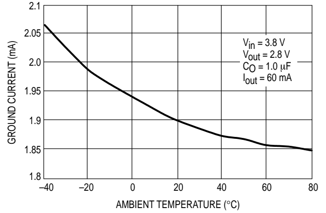
Figure 2. Ground Current versus Ambient Temperature
