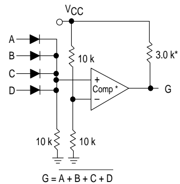
Figure 17. NOR Gate
