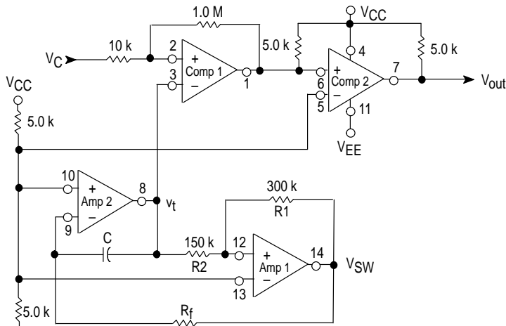
Figure 11. Pulse Width Modulator Schematic and Waveforms
