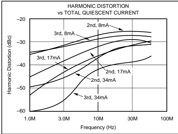
FIGURE 5. Harmonic Distortion.
