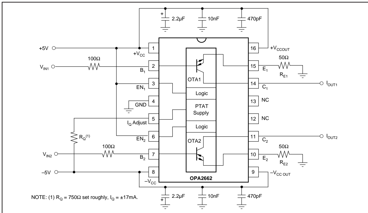
FIGURE 6. Basic Connections.
