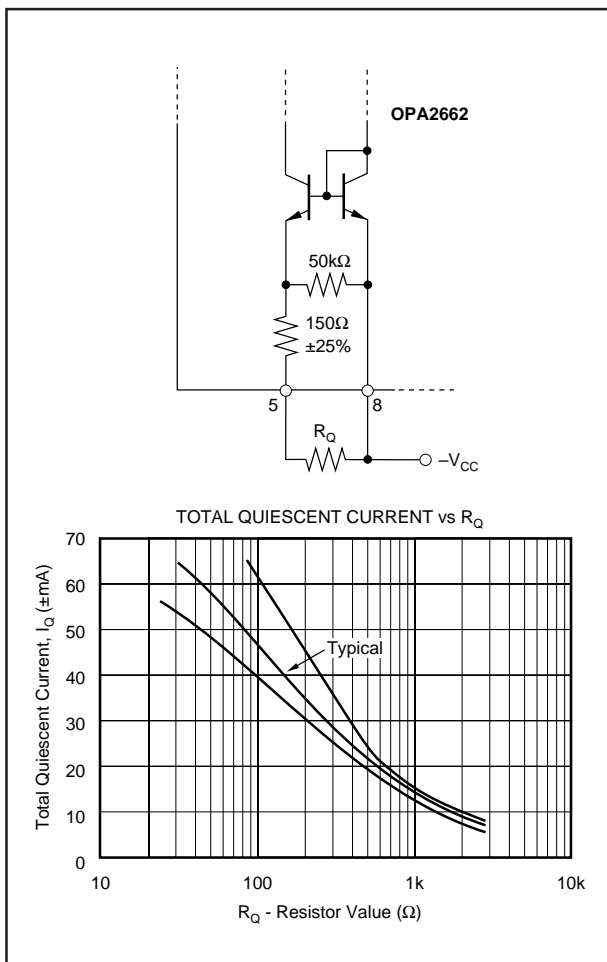
FIGURE 7. Quiescent Current Setting.
