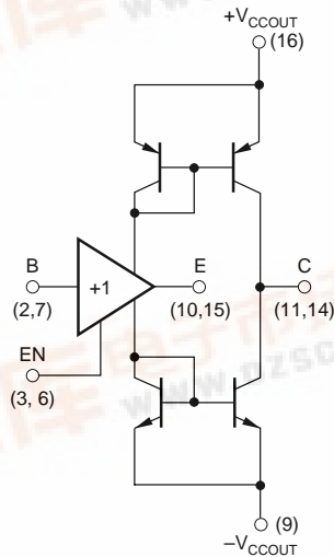
1/2 OPA2662
