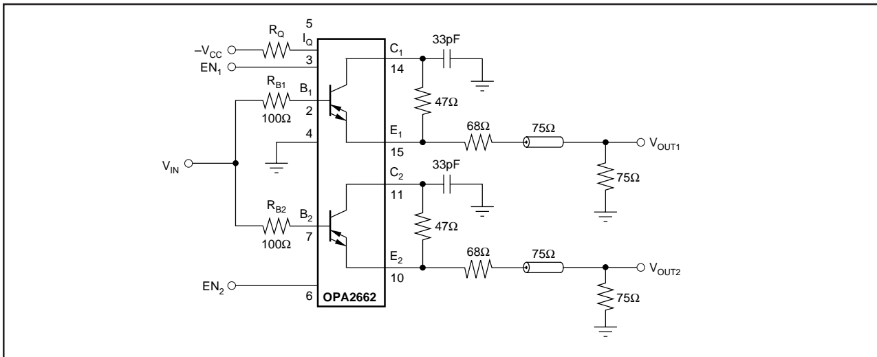
FIGURE 14. Direct Feedback Buffer and 1 to 2 Demultiplexer.
