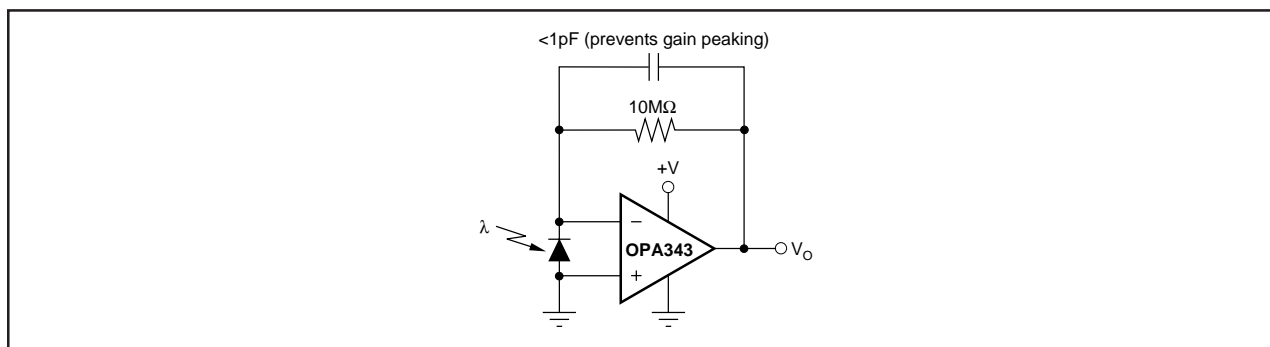
FIGURE 8. Transimpedance Amplifier.
