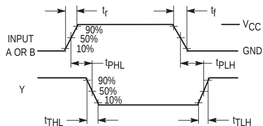
Figure 1. Switching Waveforms
