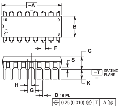
PDIP-16 N SUFFIX CASE 648-08 ISSUE R
