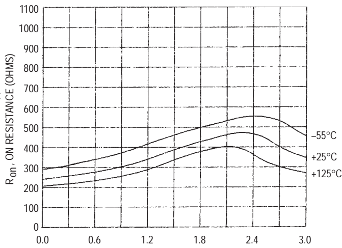
Figure 6. Typical On Resistance V CC = 3V
