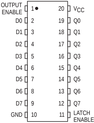
PIN ASSIGNMENT
