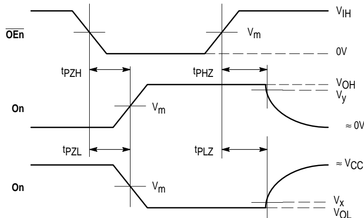
WAVEFORM 2 - OUTPUT ENABLE AND DISABLE TIMES t_R = t_F = 2.0\text{ns} , 10% to 90%; f = 1\text{MHz} ; t_{WJ} = 500\text{ns}
