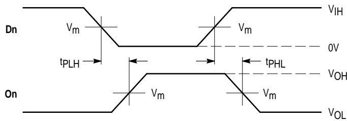
WAVEFORM 1 - PROPAGATION DELAYS t_R = t_F = 2.0\text{ns} , 10% to 90%; f = 1\text{MHz} ; t_{WJ} = 500\text{ns}
