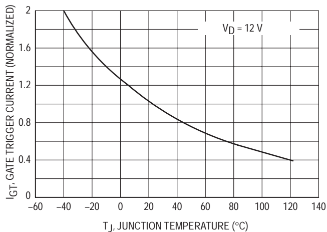
Figure 6. Typical Gate Trigger Current versus Temperature
