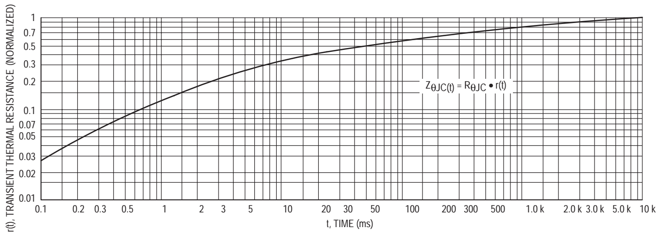
Figure 5. Thermal Response
