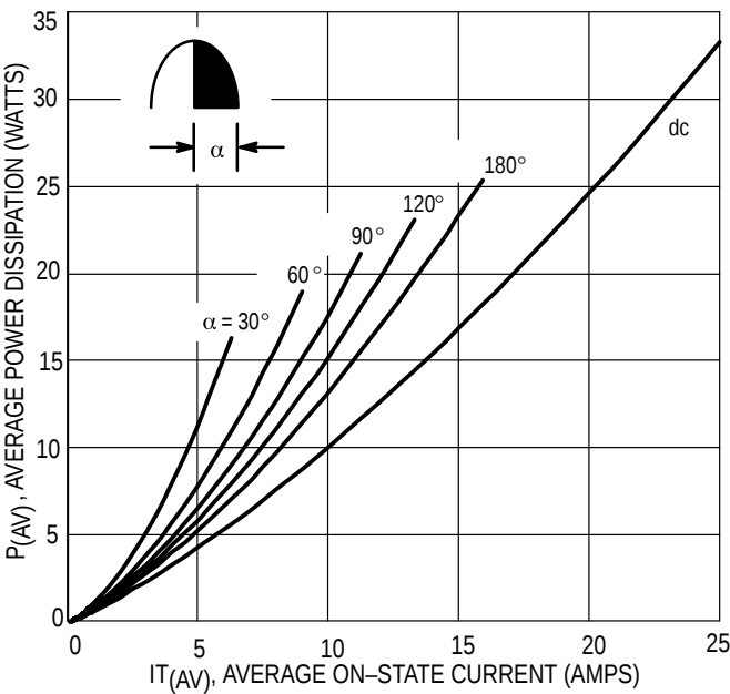
Figure 2. Maximum On-State Power Dissipation
