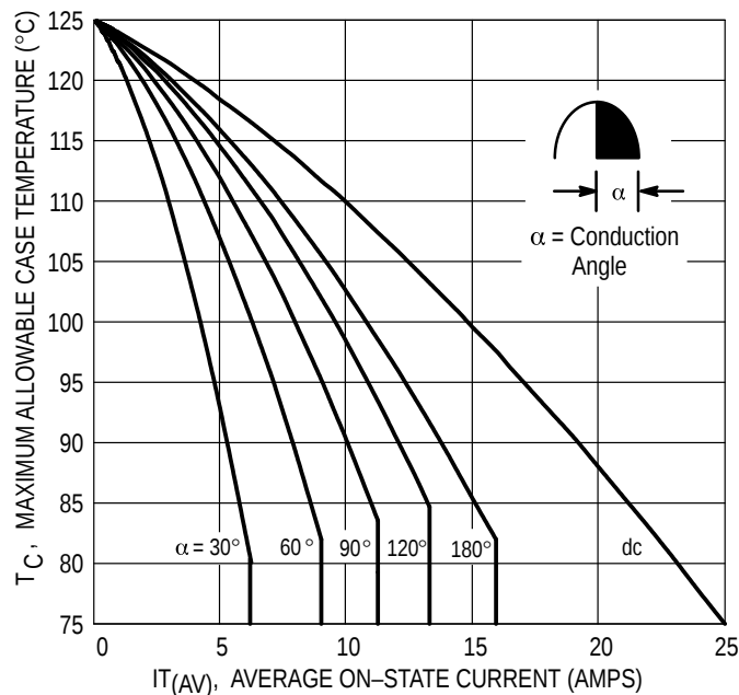
Figure 1. Average Current Derating
