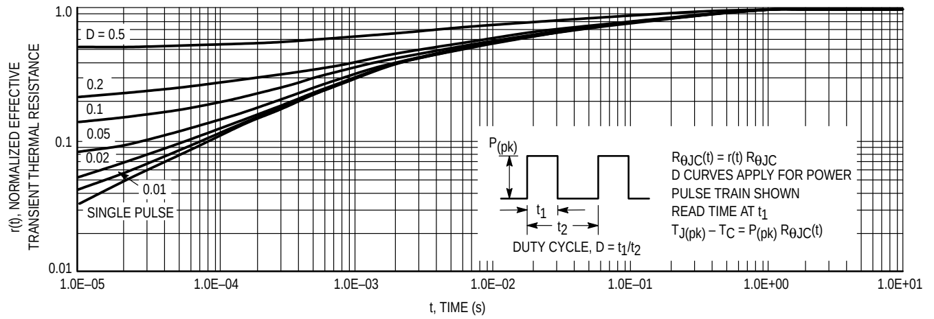
Figure 12. Thermal Response
