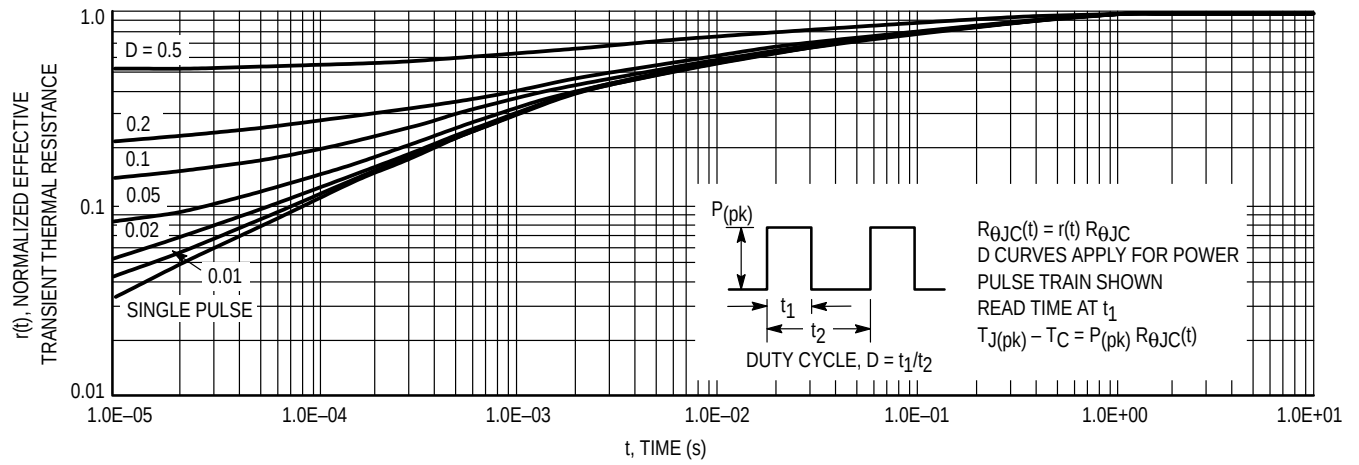
Figure 11. Thermal Response
