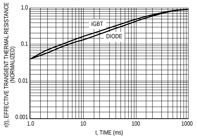
Figure 18. Thermal Response
