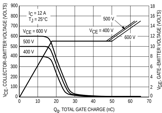
Figure 6. Collector-Emitter and Gate-Emitter Voltages versus Total Gate Charge
