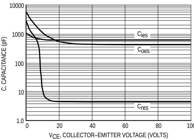
Figure 15. Capacitance Variation
