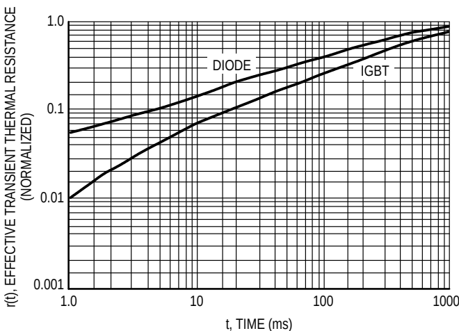
Figure 17. Thermal Response
