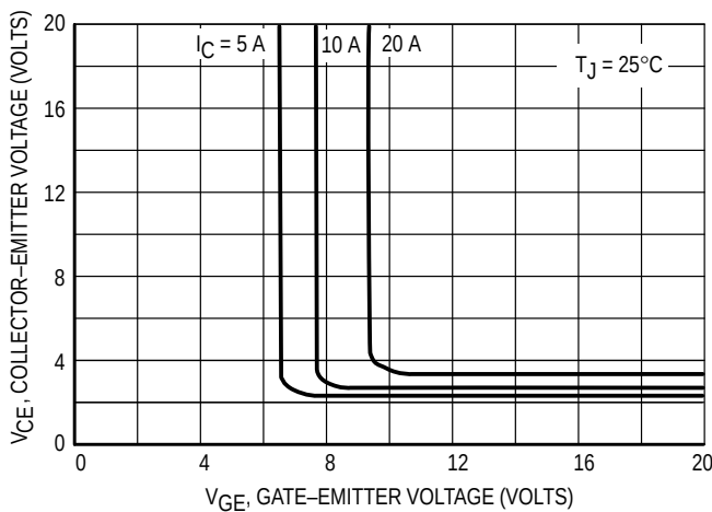
Figure 5. Collector-Emitter Voltage versus Gate-Emmitter Voltage
