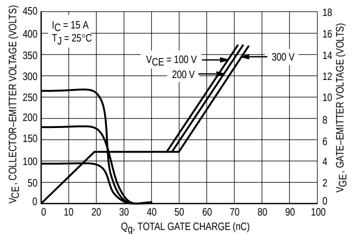
Figure 6. Collector-Emitter and Gate-Emmitter Voltages versus Total Gate Charge
