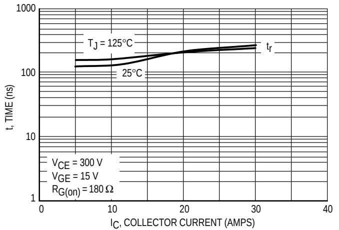
Figure 10. Inductive Switching Times versus Collector Current
