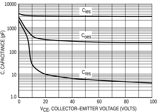
Figure 14. Capacitance Variation
