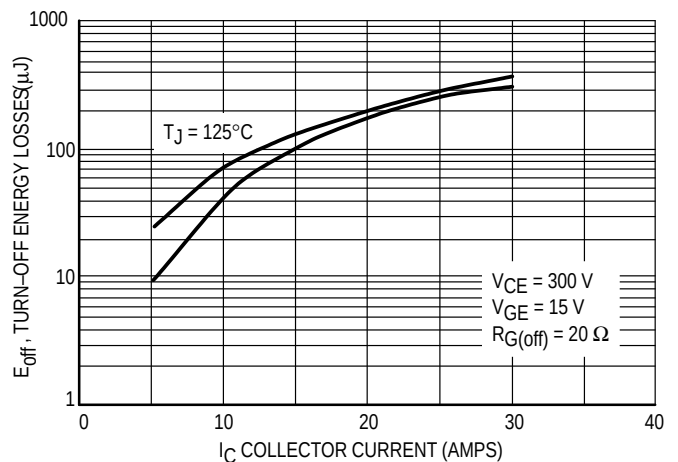
Figure 12. Turn-Off Energy Losses versus Collector Current
