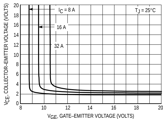
Figure 5. Collector-Emmitter Voltage versus Gate-Emmitter Voltage
