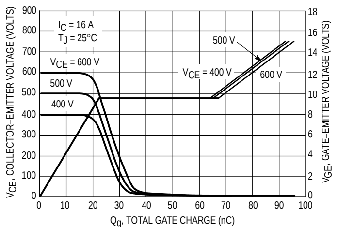
Figure 6. Collector-Emmitter and Gate-Emmitter Voltages versus Total Gate Charge
