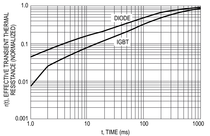
Figure 18. Thermal Response
