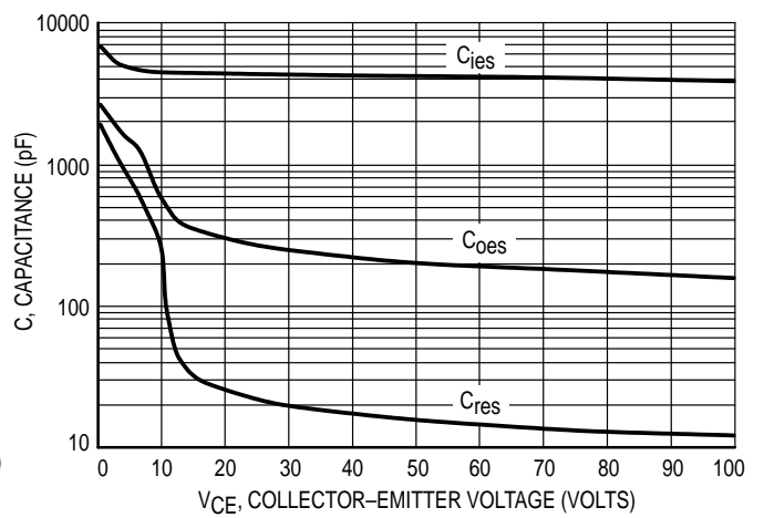
Figure 16. Capacitance Variation
