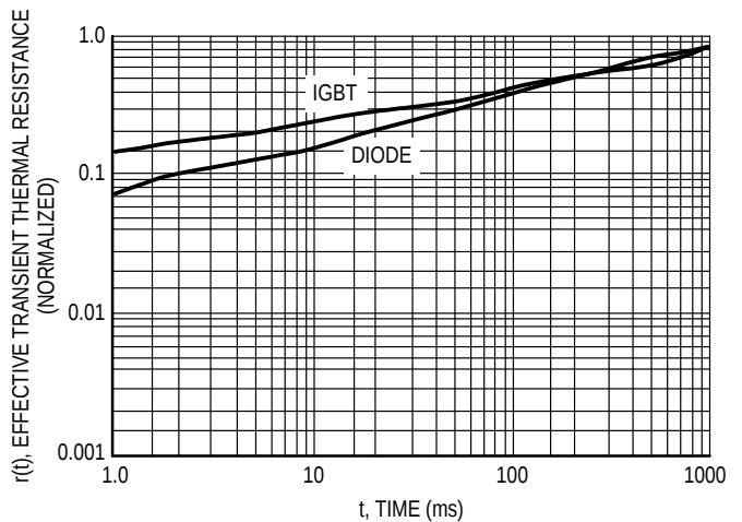
Figure 18. Thermal Response
