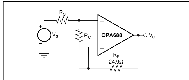
FIGURE 6. Unity-Gain Buffer.
