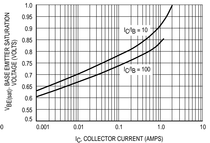
Figure 4. Base Emitter Saturation Voltage versus Collector Current
