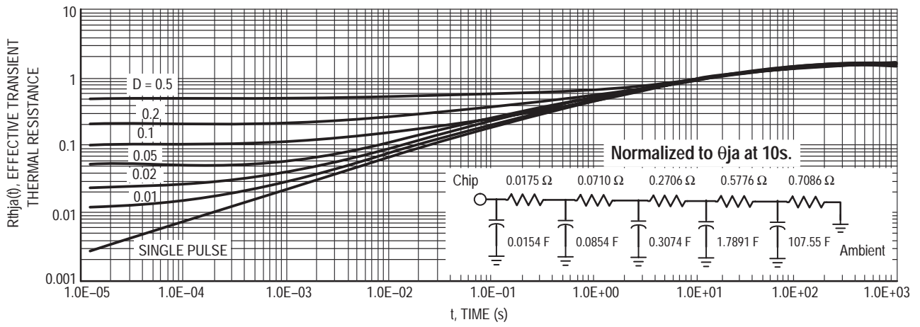
Figure 14. Thermal Response
