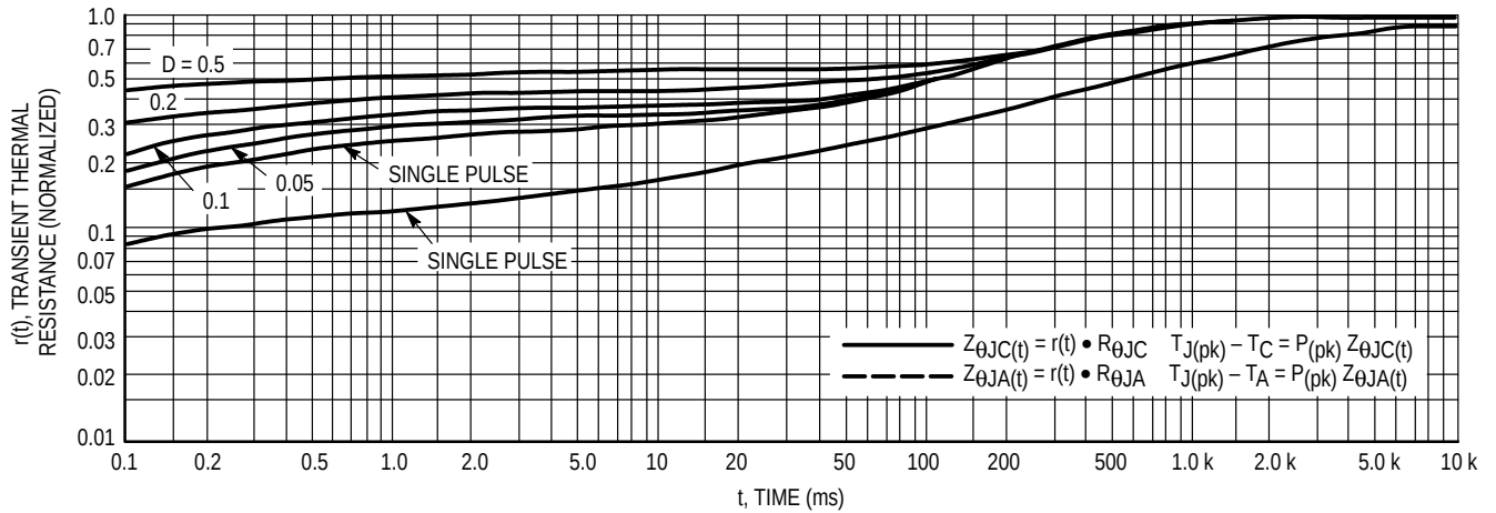
Figure 12. Thermal Response
