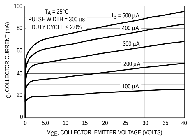
Figure 10. Collector Characteristics
