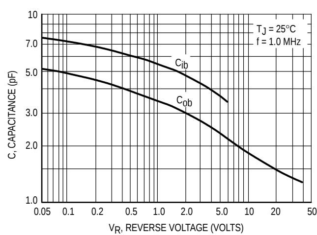
Figure 16. Capacitance
