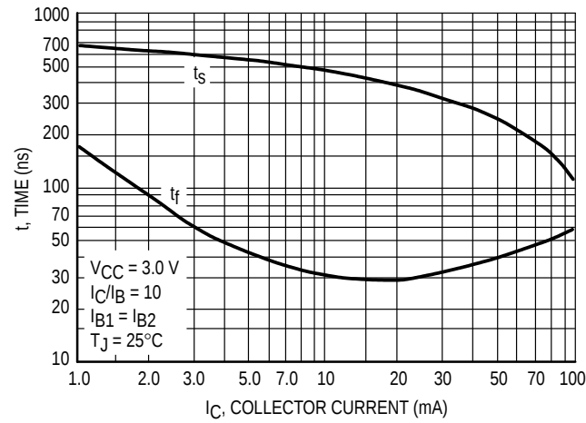
Figure 14. Turn-Off Time
