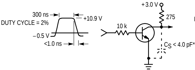
Figure 1. Turn–On Time
